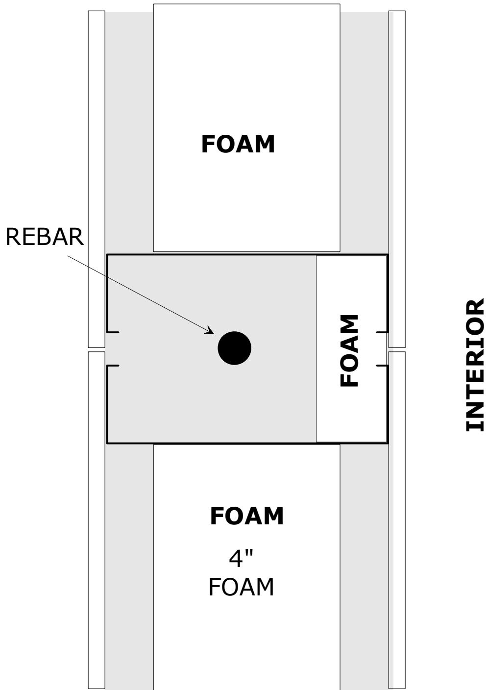
PLAN VIEW
