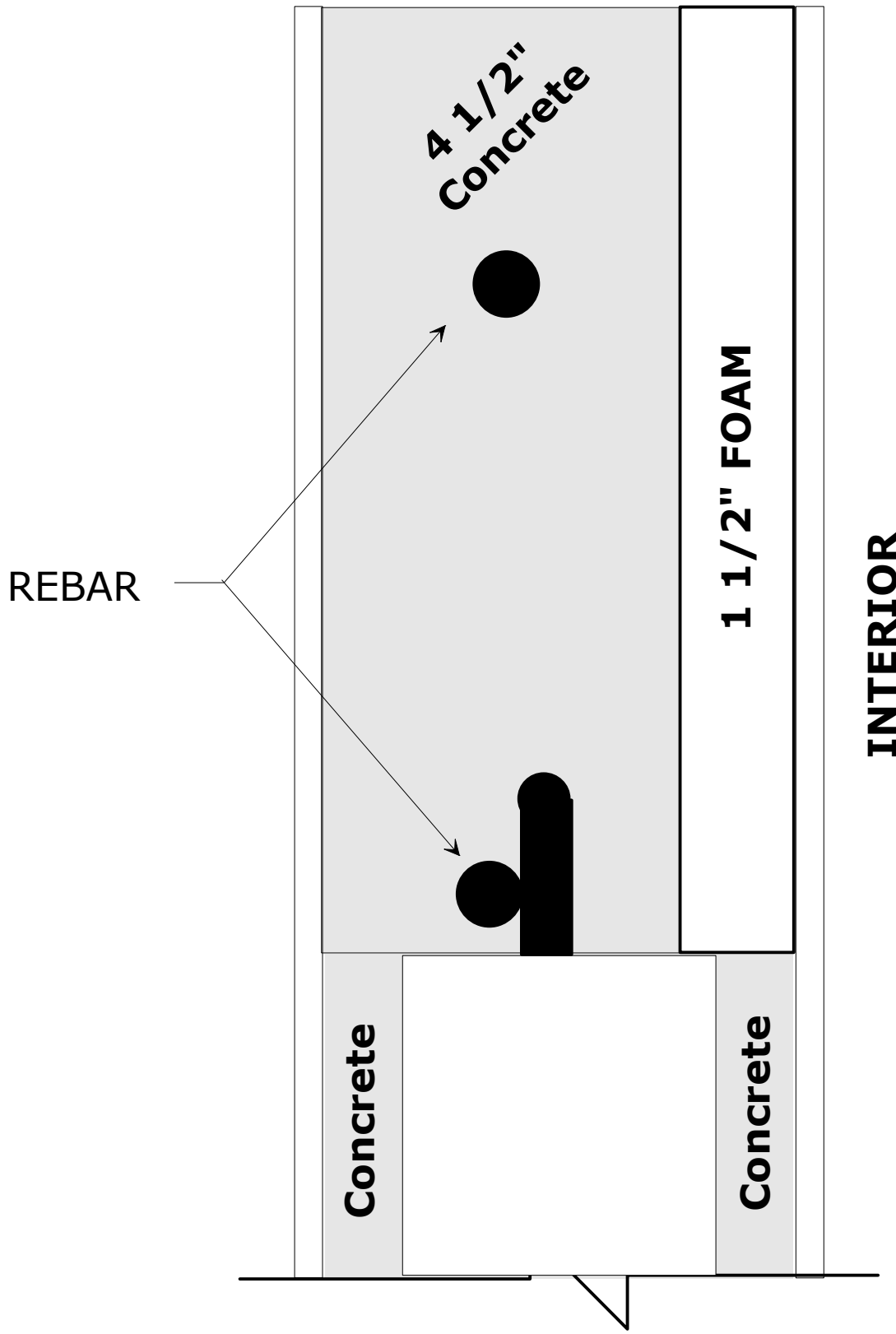
SECTION VIEW
